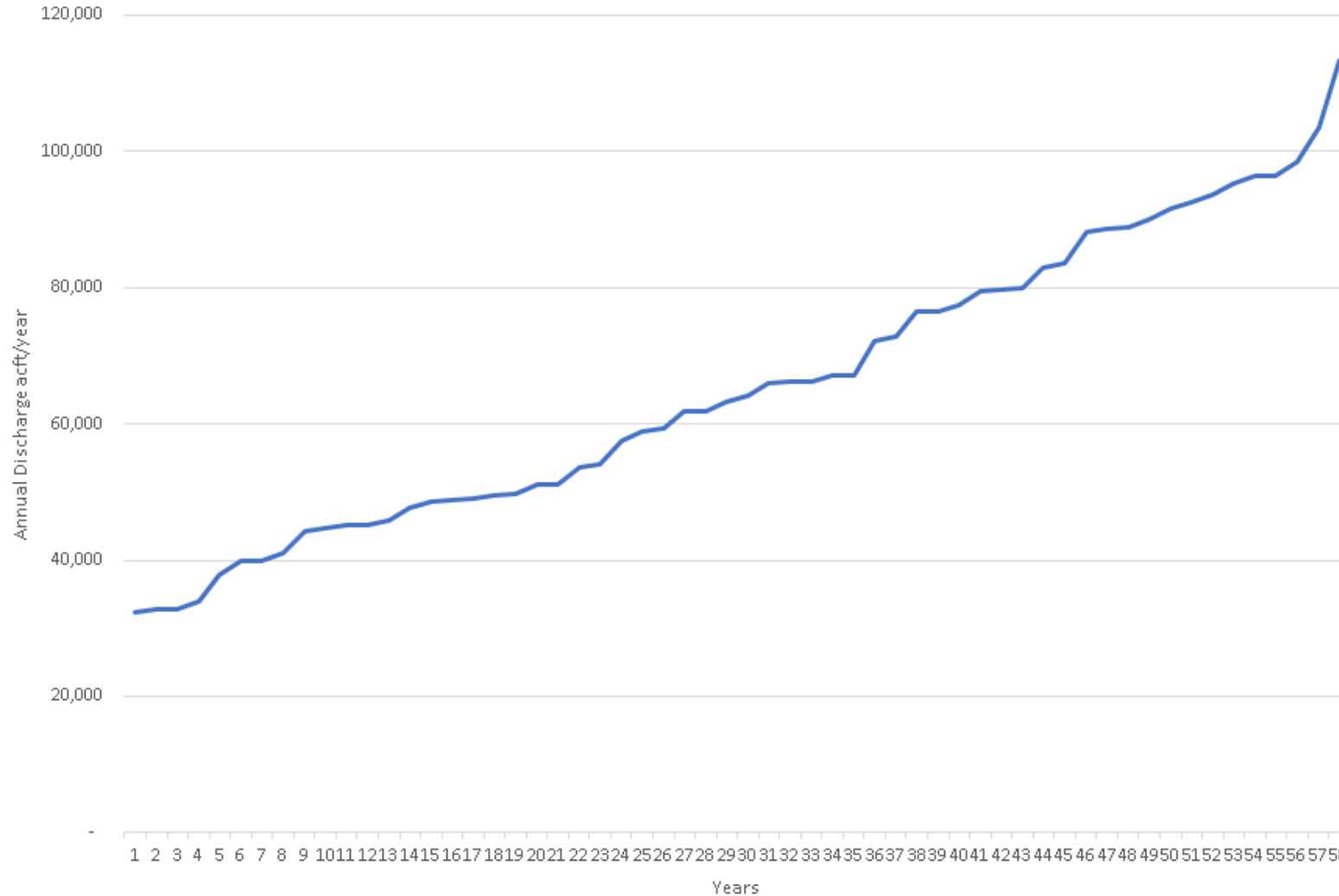
Figure AA Whitewater River Near Mecca 1961-2018 Annual Discharge acft/yr
