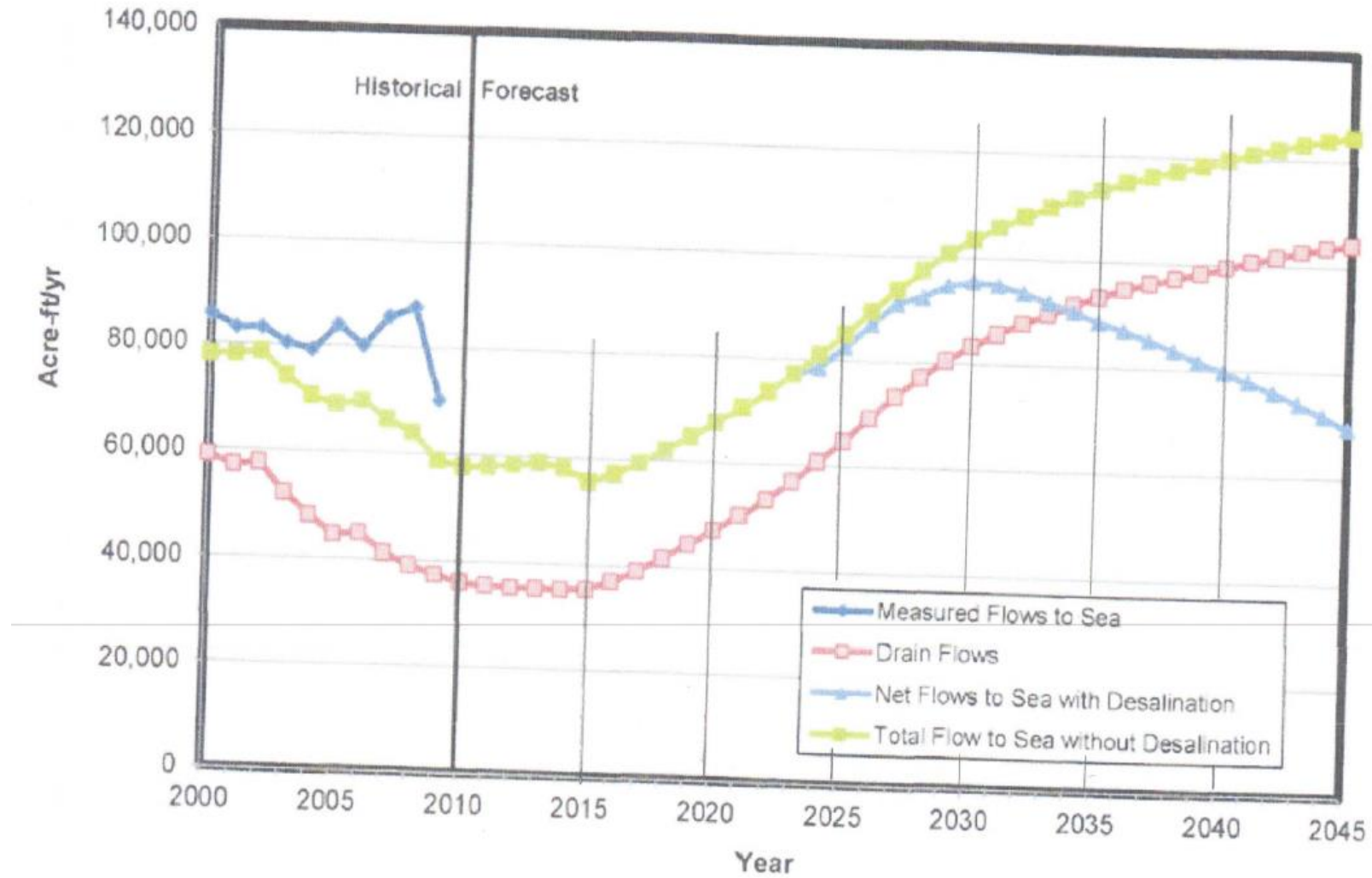
Figure 7-5 Historical and Projected Drain Flows
